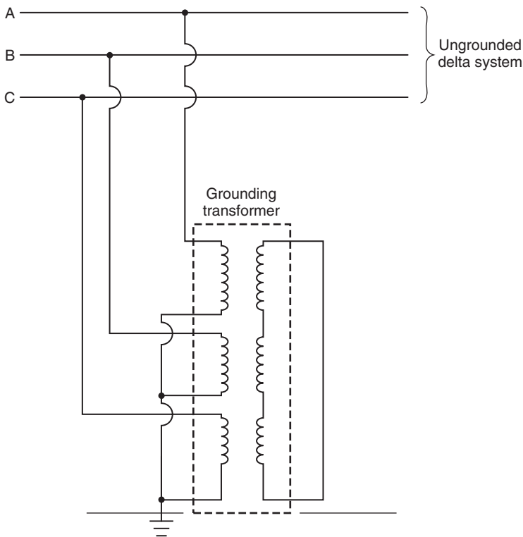
FIGURE 10.6 Grounded wye-delta transformer used to derive a system ground.
