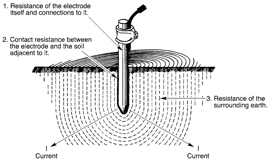
FIGURE 4.14 Components of earth resistance in an earth electrode. (Courtesy of AVO Training Institute, Inc.)
