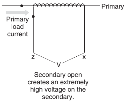
FIGURE 10.3 Open circuit on secondary of current transformer.
