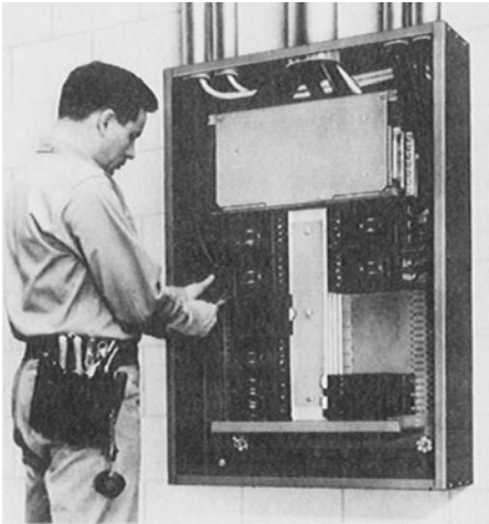
FIGURE 3.13 Panelboards equipped with molded-case circuit breakers. (Courtesy McGraw-Hill, Inc.)
