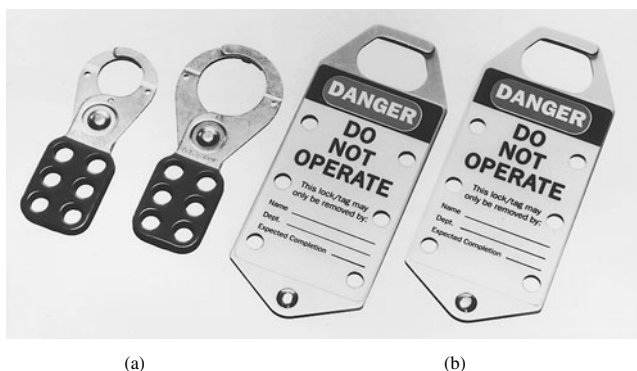
FIGURE 2.55 Multiple-lock devices. (Courtesy Ideal Industries, Inc.)
