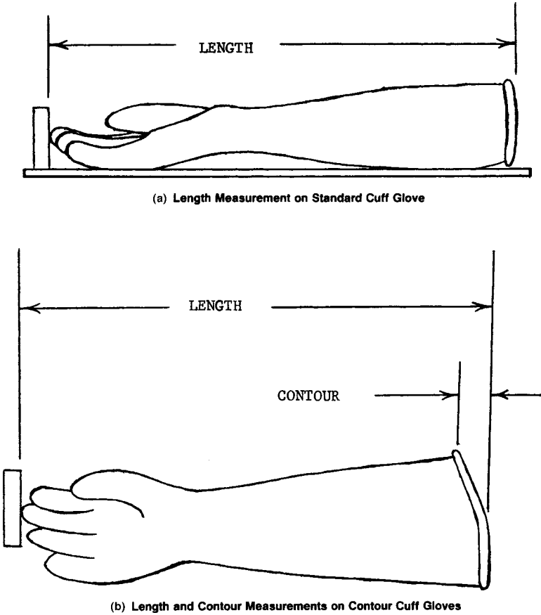
FIGURE 2.14 Dimension measurements for standard and contour cuff rubber gloves. (Courtesy ASTM.)
