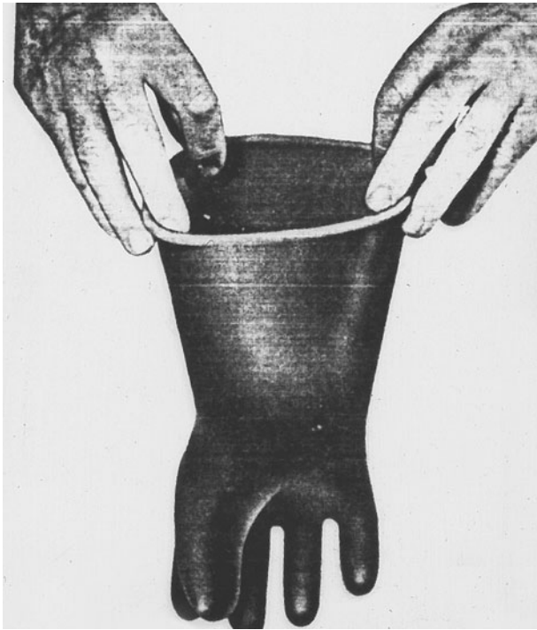
FIGURE 2.22 Inflating rubber gloves by twirling. (a) Grasping; (b) stretching; (c) twirling. ( Courtesy ASTM. )
